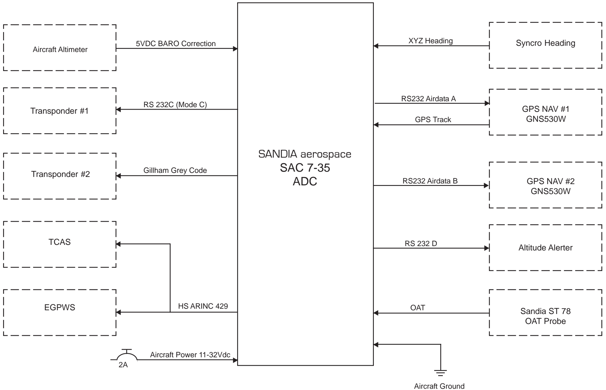
Typical SAC 7-35 Interface with Garmin 400W/500W
